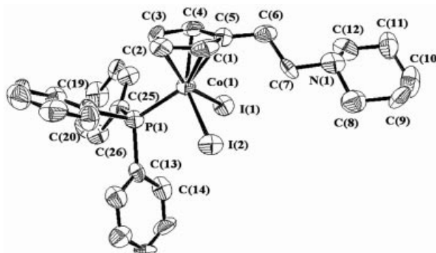
Figure 6. ORTEP diagram of 13 with the probability ellipsoids drawn at the 50% level. Hydrogen atoms, dichloromethane solvate molecule and iodide anion have been omitted for clarity. Selected bond lengths [ \text{\AA} ] and angles [ ^\circ ]: Average Co–C(ring) 2.094(11) , Co(1)–P(1) 2.239(5) , Co(1)–I(1) 2.592(3) , Co(1)–I(2) 2.568(2) , average C–C(ring) 1.40(2) , N(1)–C(7) 1.488(19) , N(1)–C(12) 1.46(2) , I(1)–Co(1)–I(2) 95.40(8) , I(1)–Co(1)–P(1) 92.79(14) , I(2)–Co(1)–P(1) 91.57(14) , Co(1)–P(1)–C(13) 118.0(5) , Co(1)–P(1)–C(19) 112.7(7) , Co(1)–P(1)–C(25) 115.2(5) .
