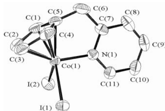
Figure 3. ORTEP diagram of 12 with the probability ellipsoids drawn at the 50% level. Hydrogen atoms have been omitted for clarity. Selected bond lengths [Å] and angles [°]: Average Co–C(ring) 2.039(8), Co(1)–N(1) 1.956(6), Co(1)–I(1) 2.5779(16), Co(1)–I(2) 2.5796(16), average C–C(ring) 1.403(14), N(1)–C(7) 1.351(10), N(1)–C(11) 1.327(10), C(7)–C(8) 1.392(12), C(8)–C(9) 1.360(14), C(9)–C(10) 1.370(14), C(10)–C(11) 1.365(12), I(1)–Co(1)–I(2) 96.68(4), I(1)–Co(1)–N(1) 95.12(18), I(2)–Co(1)–N(1) 95.12(19), Co(1)–N(1)–C(7) 116.9(5).
