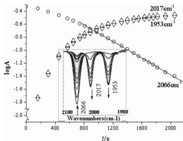
Figure 5. Reduction of diiodocarbonyl- \eta^5 -(2-piperidinyethyl)cyclopentadienylcobalt(III) by carbon monoxide released via its own chelation. The inset IR spectra show the reducing \nu(\text{CO}) of 6' at 2066 \text{cm}^{-1} and the increasing \nu(\text{CO}) of 6 at 2017 and 1953 \text{cm}^{-1} , respectively.
