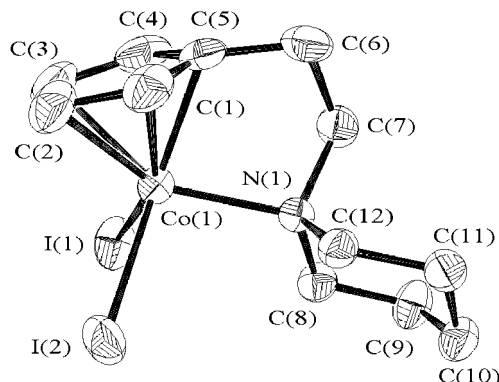
Figure 2. ORTEP diagram of 10 with the probability ellipsoids drawn at the 50% level. Hydrogen atoms have been omitted for clarity. Selected bond lengths [Å] and angles [°]: Average Co–C(ring) 2.055(6), Co(1)–N(1) 2.097(3), Co(1)–I(1) 2.6015(7), Co(1)–I(2) 2.5714(8), average C–C(ring) 1.4084(6), I(1)–Co(1)–I(2) 92.70(2), I(1)–Co(1)–N(1) 100.32(8), I(2)–Co(1)–N(1) 96.34(9), Co(1)–N(1)–C(7) 104.1(2).
