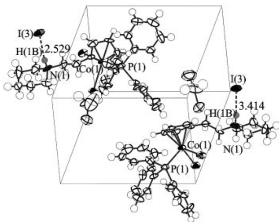
Figure 7. N–H⋯I hydrogen bonding in the unit cell of complex 13 .
