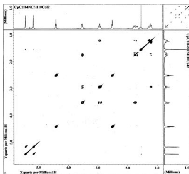
Figure 4. COSY spectrum of diiodo- \eta^5:\eta^1 -(2-piperidinoethyl)cyclopentadienylcobalt(III) ( \text{C}_5\text{H}_4\text{C}_2\text{H}_4\text{N}_3\text{H}_{10}\text{CoI}_2 ) ( 10 ) in \text{CDCl}_3 at 25 °C.
