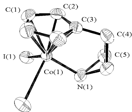
Figure 1. ORTEP diagram of 9 with the probability ellipsoids drawn at the 50% level. Hydrogen atoms have been omitted for clarity. Selected bond lengths [Å] and angles [°]: Average Co–C(ring) 2.045(1), Co(1)–N(1) 1.979(8), Co(1)–I(1) 2.5979(10), Average C–C(ring) 1.4054(4), I(1)–Co(1)–I(1A) 1 96.50(5), I(1)–Co(1)–N(1) 92.07(16), I(1A)–Co(1)–N(1) 92.07(16), Co(1)–N(1)–C(5) 110.3(7).
